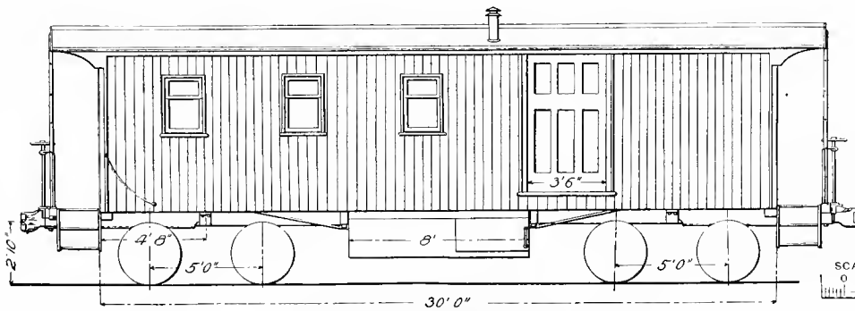
Fig. 85. Side Elevation.
